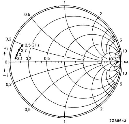
Fig. 16 Optimum load impedance as a function of frequency.
