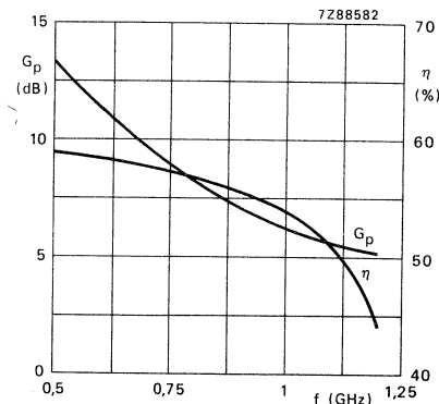
Fig. 17 Power gain and efficiency as a function of frequency.
