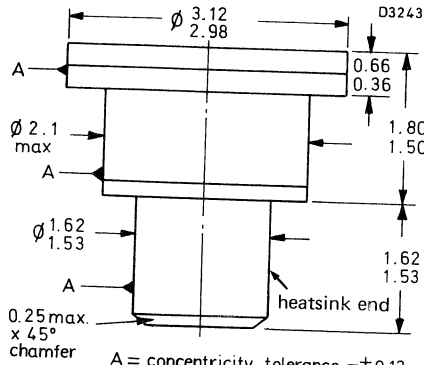
case style SOD-45
