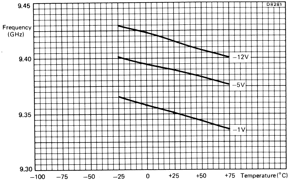
Typical output frequency as a function of temperature at three tuning voltages.
