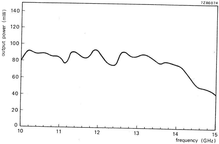
Fig. 6 Typical test curve of YG1104.
