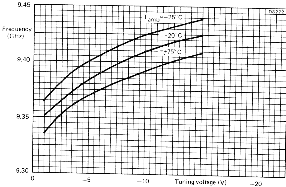
Typical output frequency as a function of tuning voltage at three ambient temperatures
