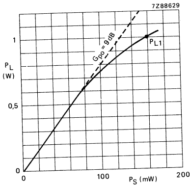
Fig. 23 Load power as a function of source power at f = 1 GHz.
