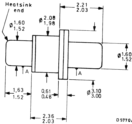
case style SOD-31
