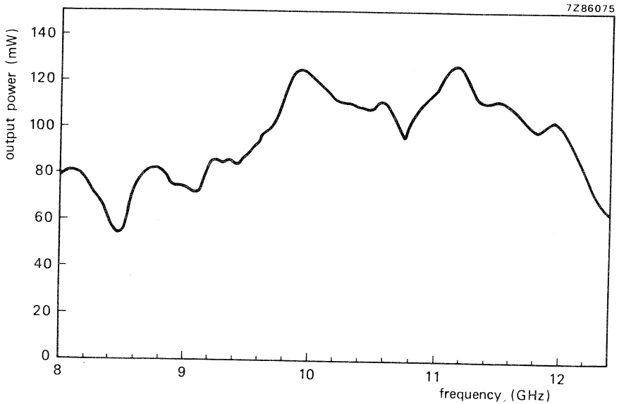
Fig. 5 Typical test curve of YG1103.
