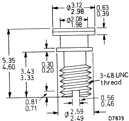
case style SOD-44
