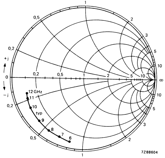
Fig. 5 Input impedance derived from input reflection coefficient s_{iS} co-ordinates in ohm \times 50 .
