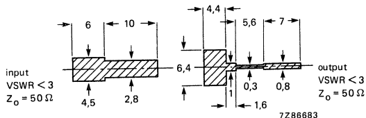
Fig. 7 Prematching test circuit boards for the PTB42002X at 4,2 GHz. (Dimensions in mm.)
