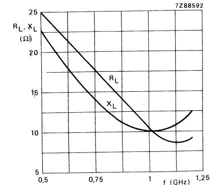
Fig. 24 Load impedance as a function of frequency. (See also Fig. 32).
