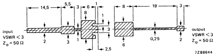
Fig. 5 Prematching test circuit boards for the PKB32003U at 3 GHz. (Dimensions in mm.)
