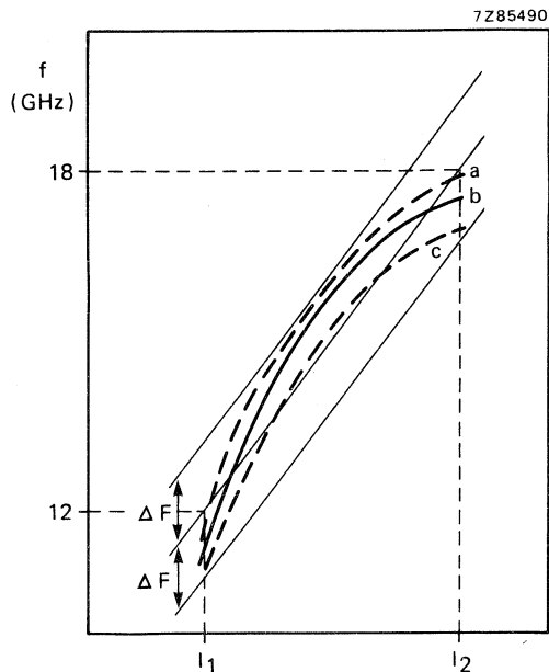
Fig. 4 Linear relation of frequency as a function of current in main coil; typical values, curve a at -40\text{ }^{\circ}\text{C} ; curve b at +25\text{ }^{\circ}\text{C} and curve c at +85\text{ }^{\circ}\text{C} . Deviation \Delta F max. \pm 50\text{ MHz} over the whole frequency range and operating temperature range. Frequency drift with temperature ( -40 to 85\text{ }^{\circ}\text{C} ) at fixed current: max. \pm 25\text{ MHz} .
