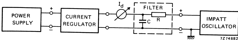
Fig. 4 Bias configuration for stable IMPATT oscillator. R = 82 \Omega (carbon resistor, 1 W), C = 220 nF (film capacitor 160 V). Power supply: 110 V, 100 mA.
