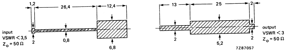
Fig. 9 Prematching test circuit board for 2 GHz. (Dimensions in mm.)
