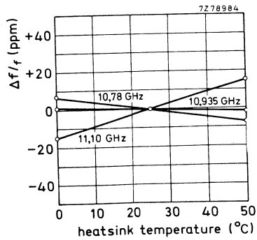
Fig. 10 Relative change of output power and frequency with heatsink temperature. V_d = 12 V.
