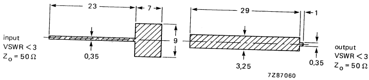
Fig. 5 Prematching test circuit board for 2 GHz. (Dimensions in mm.)
