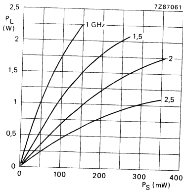
Fig. 6 Load power as a function of source power with frequency as parameter.
