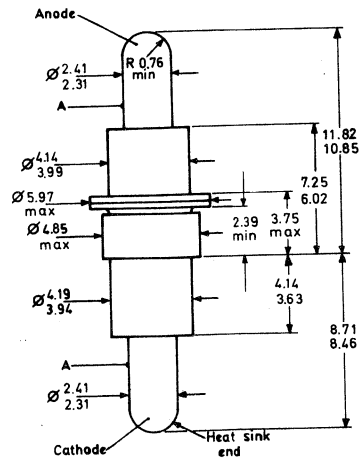
Outline drawing of 1N5153 Conforms to SOD-43
