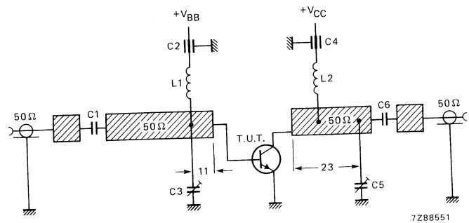
Fig. 9 Class-A test circuit at f = 1 \text{ GHz} . (Dimensions in mm.)
