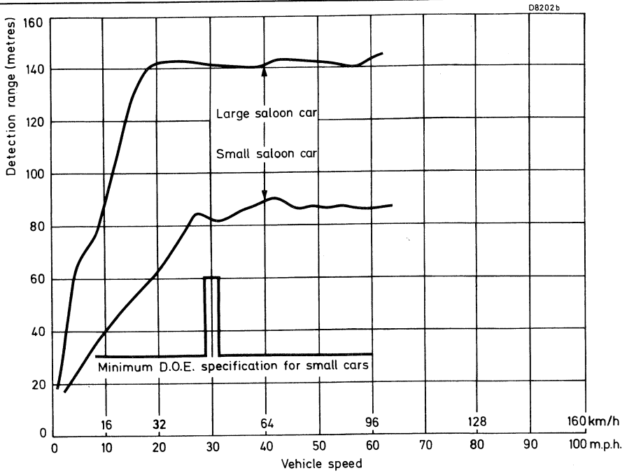
Fig.2 Typical detection curves obtained from road tests using six different microwave vehicle detectors.
