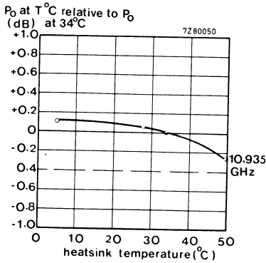
Fig. 12 Relative change of output power and frequency with heatsink temperature. I_d = 55 mA.
