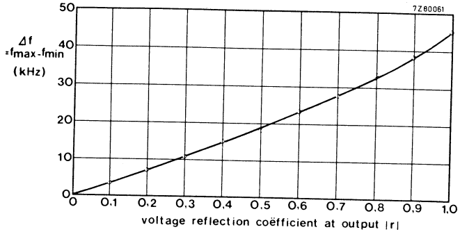
Fig. 11 Frequency pulling of the IMPATT oscillator as a function of the modulus of the voltage reflection coefficient. (Output via isolator and OSM connector.) I_d = 55 mA, f_o = 11 GHz, P_o = 110 mW.
