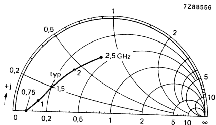
Fig. 10 Input impedance as a function of frequency for P_{L1} .
