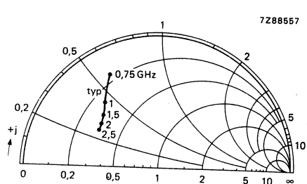
Fig. 11 Optimum load impedance as a function of frequency for P_{L1} .
