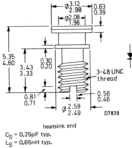
case style SOD-44
