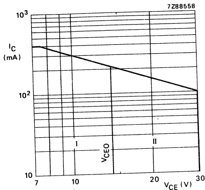
(1) Second breakdown limit (independent of temperature).
