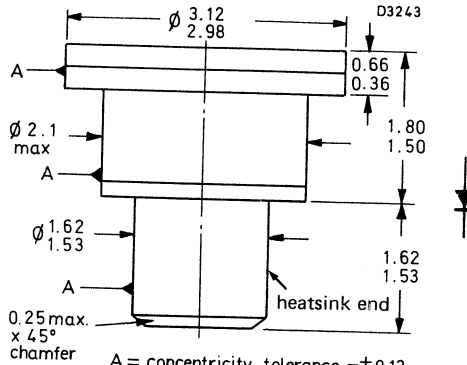
case style SOD-45
