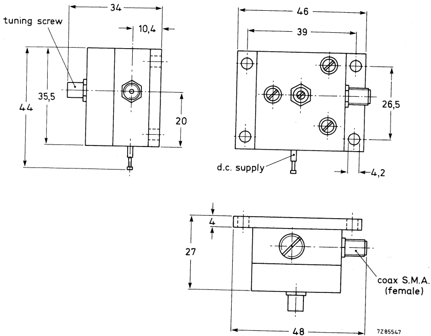
Fig. 1 Dielectric resonator stabilized Gunn oscillator.
