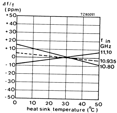
Fig. 12 Relative change of output power and frequency with heatsink temperature. I_d = 55 mA.
