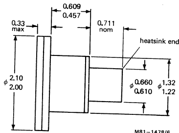
case style MO-72
