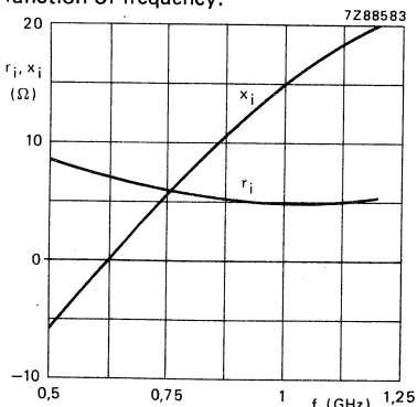
Fig. 18 Input impedance as a function of frequency. (See also Fig. 31).
