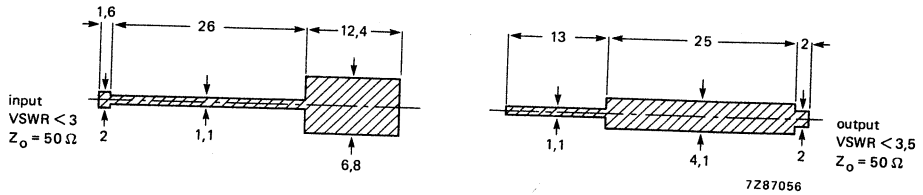
Fig. 6 Prematching test circuit board for 2 GHz. (Dimensions in mm.)
