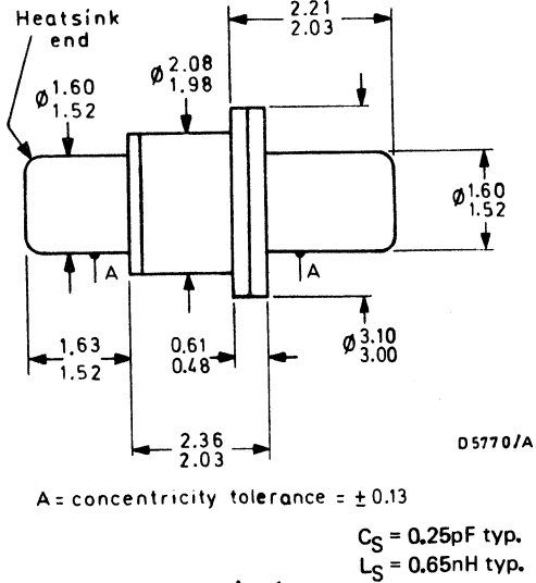
case style SOD-31 conforms to BS3934 SO-86
