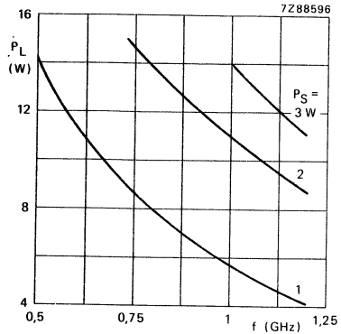
Fig. 26 Load power as a function of frequency.
