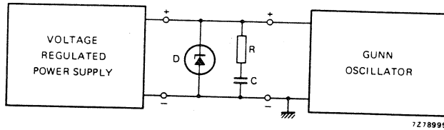
Fig. 3 Bias configuration for stable Gunn oscillator. D = voltage regulator diode, e.g. BZX70-C15; R = 1 to 10 \Omega , carbon resistor; C = 0,47 \mu F, film capacitor; Power supply up to 15 V, min. 1 A.
